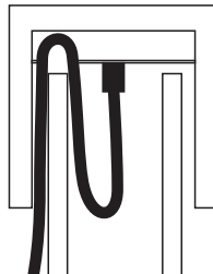
Fig. 10 b: Cross section of the plinth Lead the cable between base and mast to the outside.
