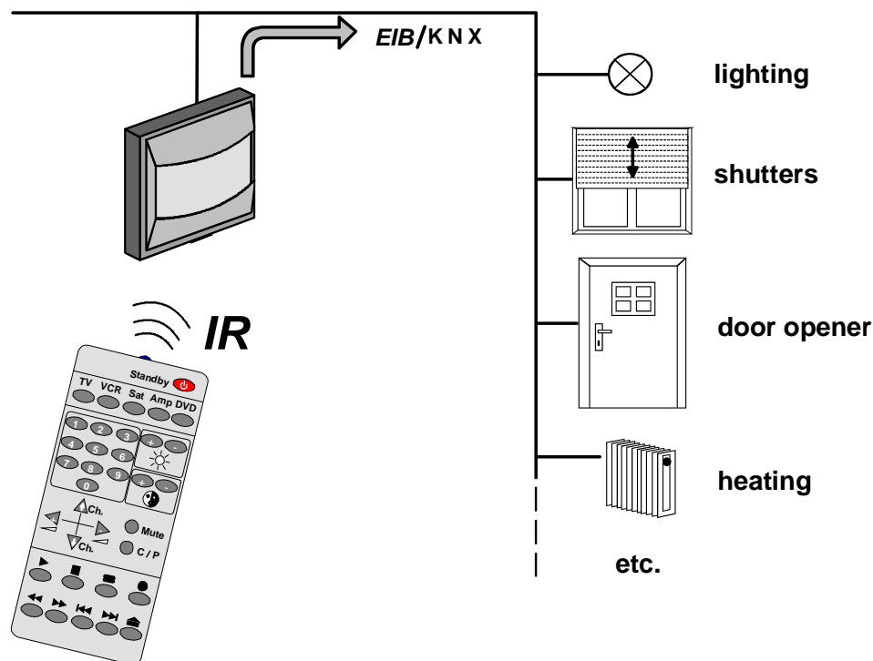
Bild 1: Controlling the existing EIB/KNX installation with an IR transmitter
